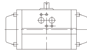
Automation (Optional) SIZE : NPS 1/2 ~ NPS 8
